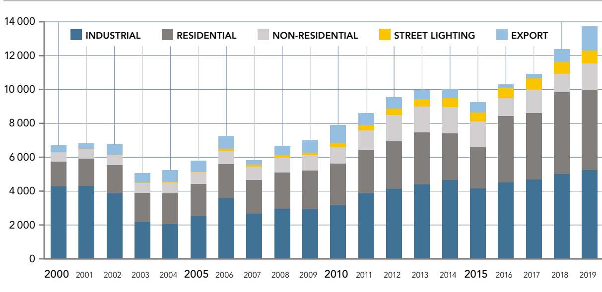
Figure 6: Utility electricity sales by customer category, including electricity export (GWh), 2000-2019
