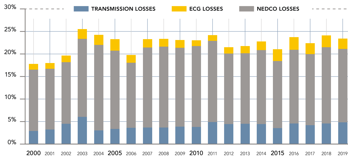
Figure 5: Transmission and distribution losses as a share of gross electricity transmitted, 2000-2019
