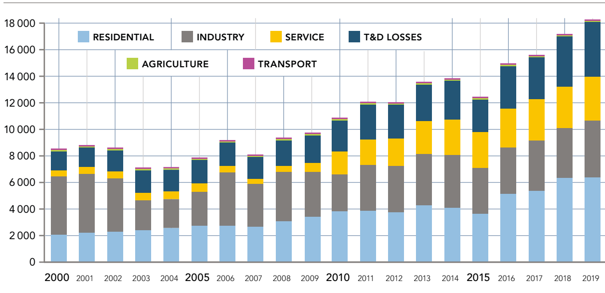
Figure 7: Electricity consumption by sector (GWh) in Ghana, including transmission and distribution losses, 2000-2019
