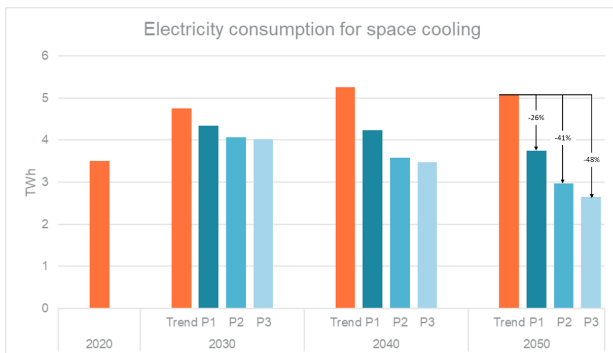
Figure 5 Mitigation prospects - Electricity consumption for space cooling 2020 - 2050
