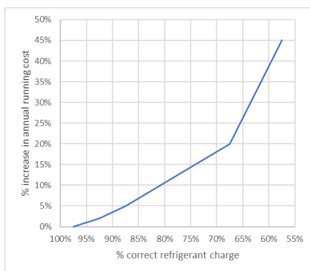
Figure 3 Relationship between Annual running costs and refrigerant leakage for small air-conditioning and commercial systems. 37
