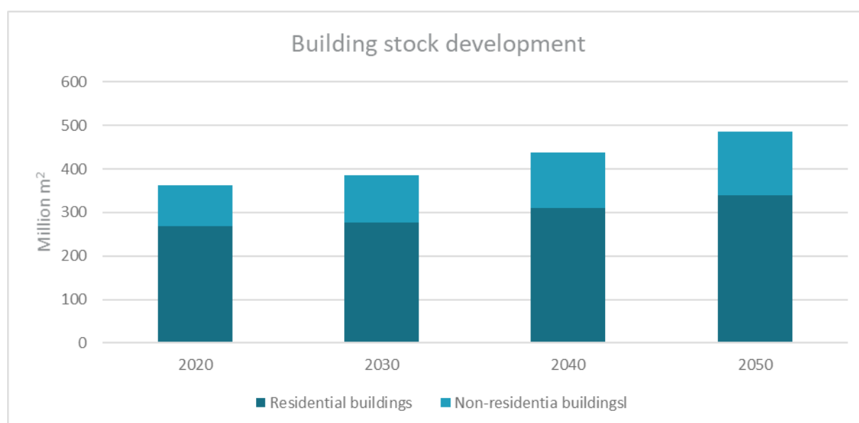
Figure 21 Building stock development 2020 - 2050
